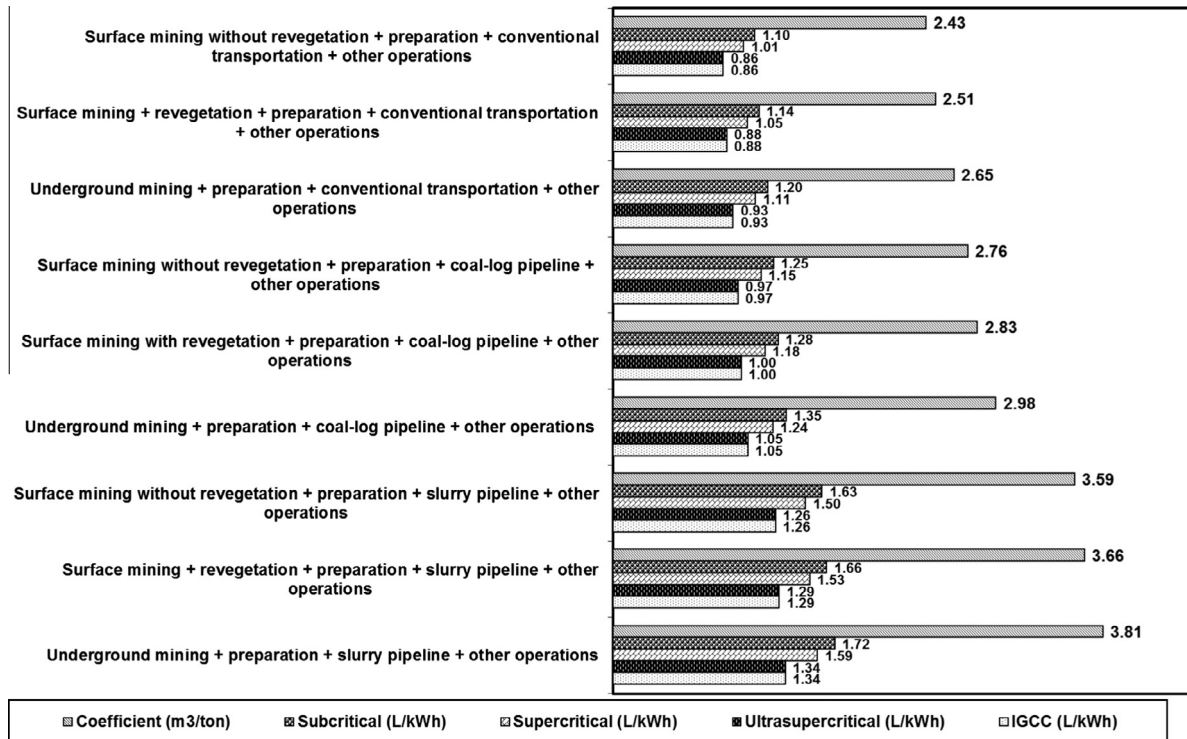
Fig. 2. Water consumption coefficients for coal upstream stage.
