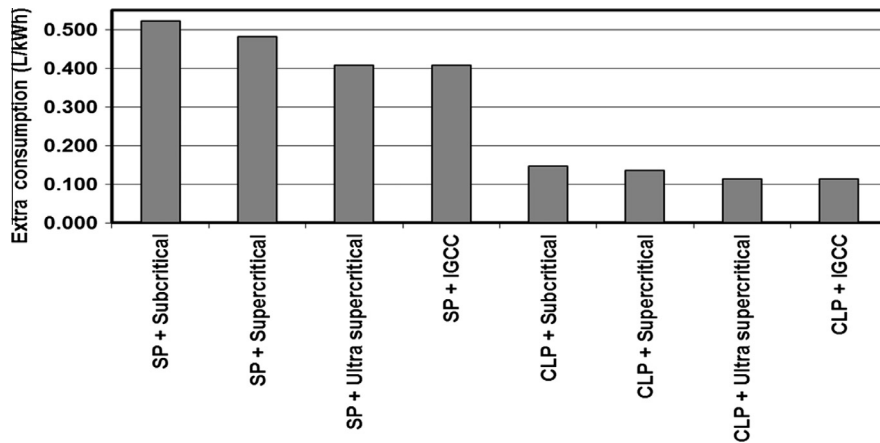
Fig. 6. Extra water-consumption coefficients resulting from changing conventional to pipeline transportation modes.
