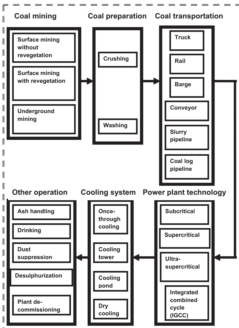
Fig. 1. System boundary and unit operations for coal-based power plants.
