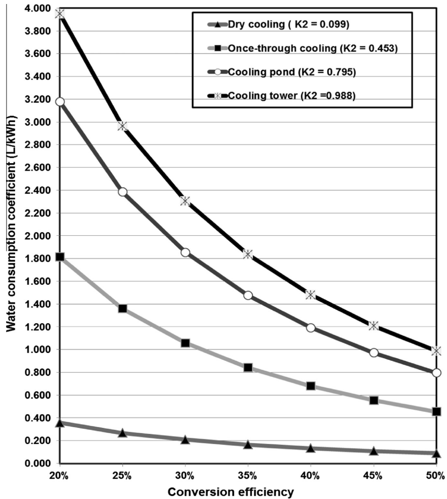
Fig. 5. Performance curves for water consumption during power generation stage.
