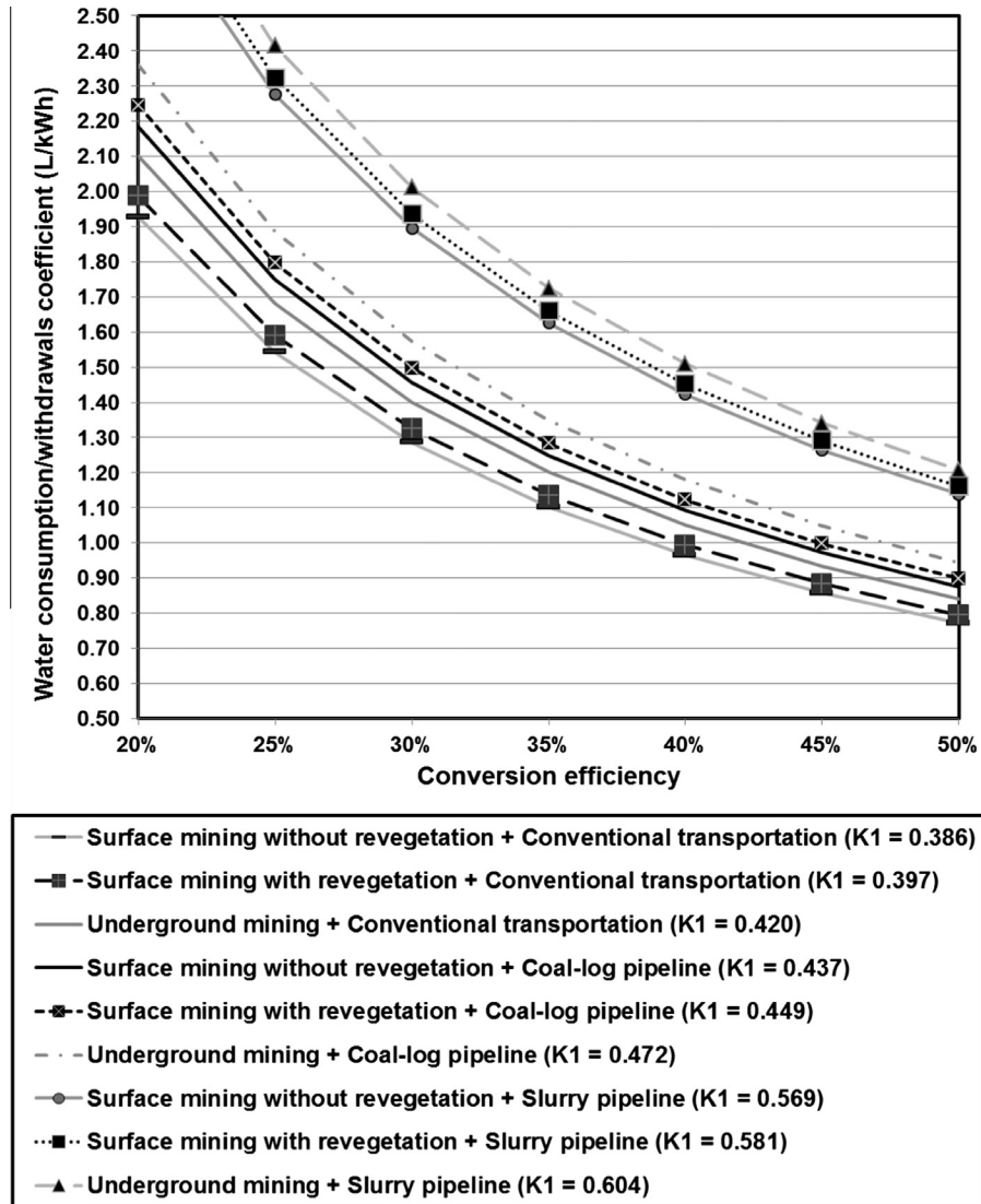
Fig. 4. Performance curves for coal upstream pathways.
