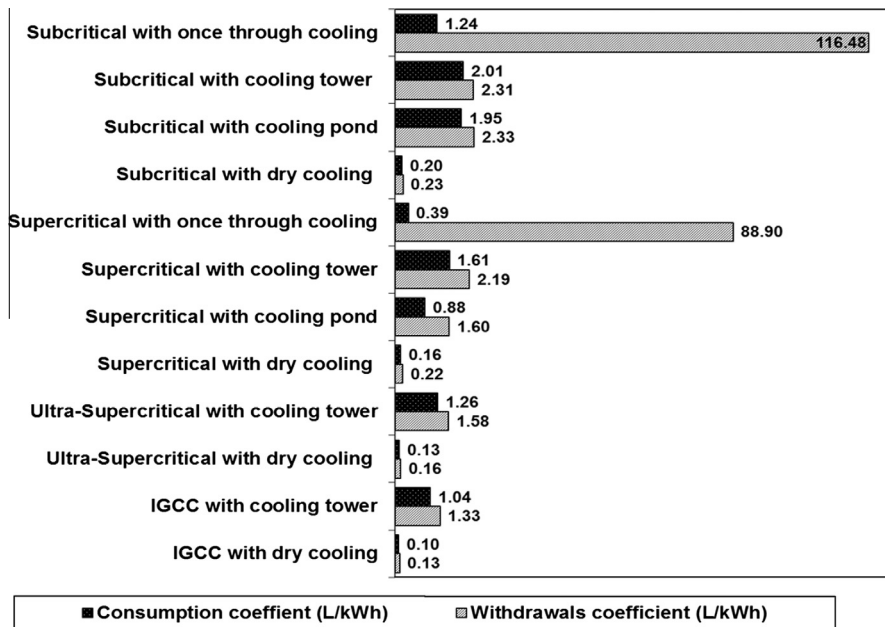
Fig. 3. Water-demand coefficients for the stage of power generation from coal.
