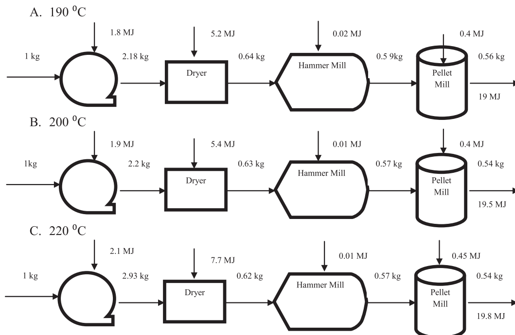
Fig. 4. Effect of change in temperature on energy and mass flow of steam pretreated pellet production.
