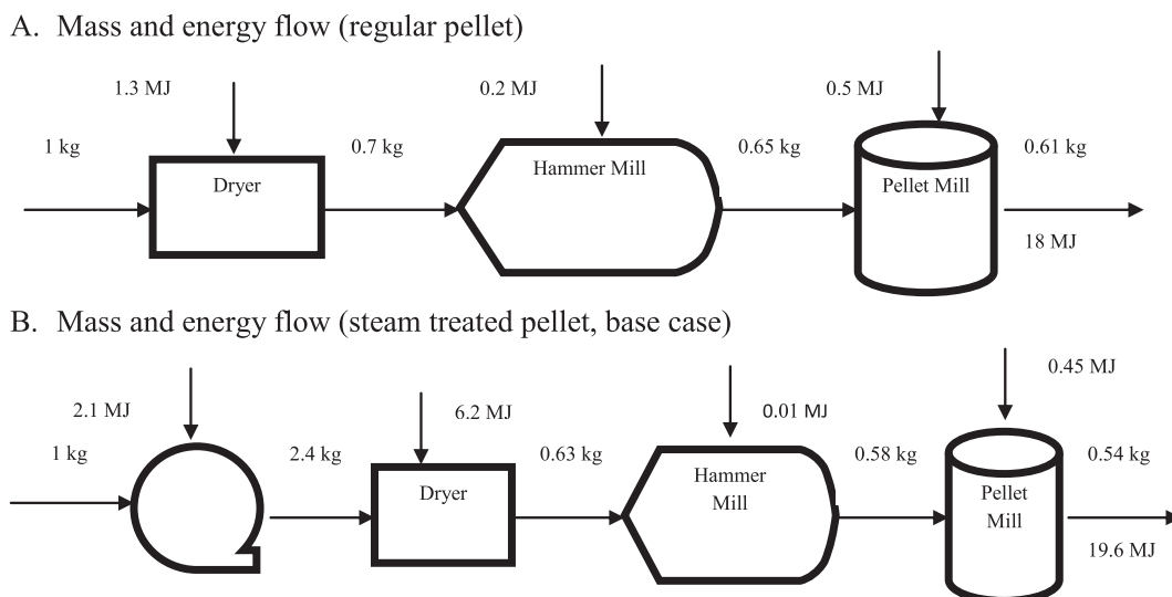
Fig. 3. Input and output energy and mass flow of regular pellet production and steam pretreated pellet production (base case).
