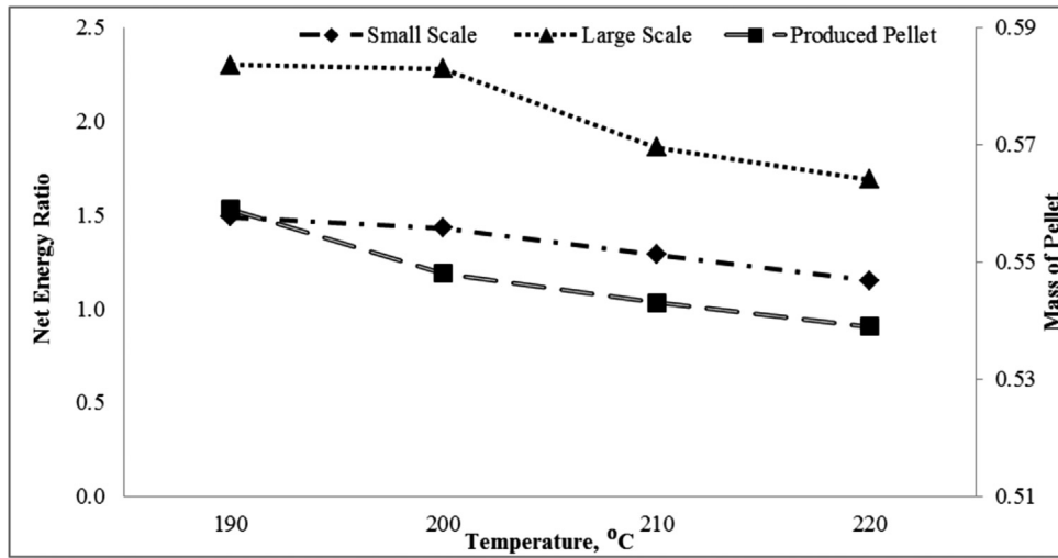
A. Variation of net energy ratio at different treatment temperatures for small and large scale cases
