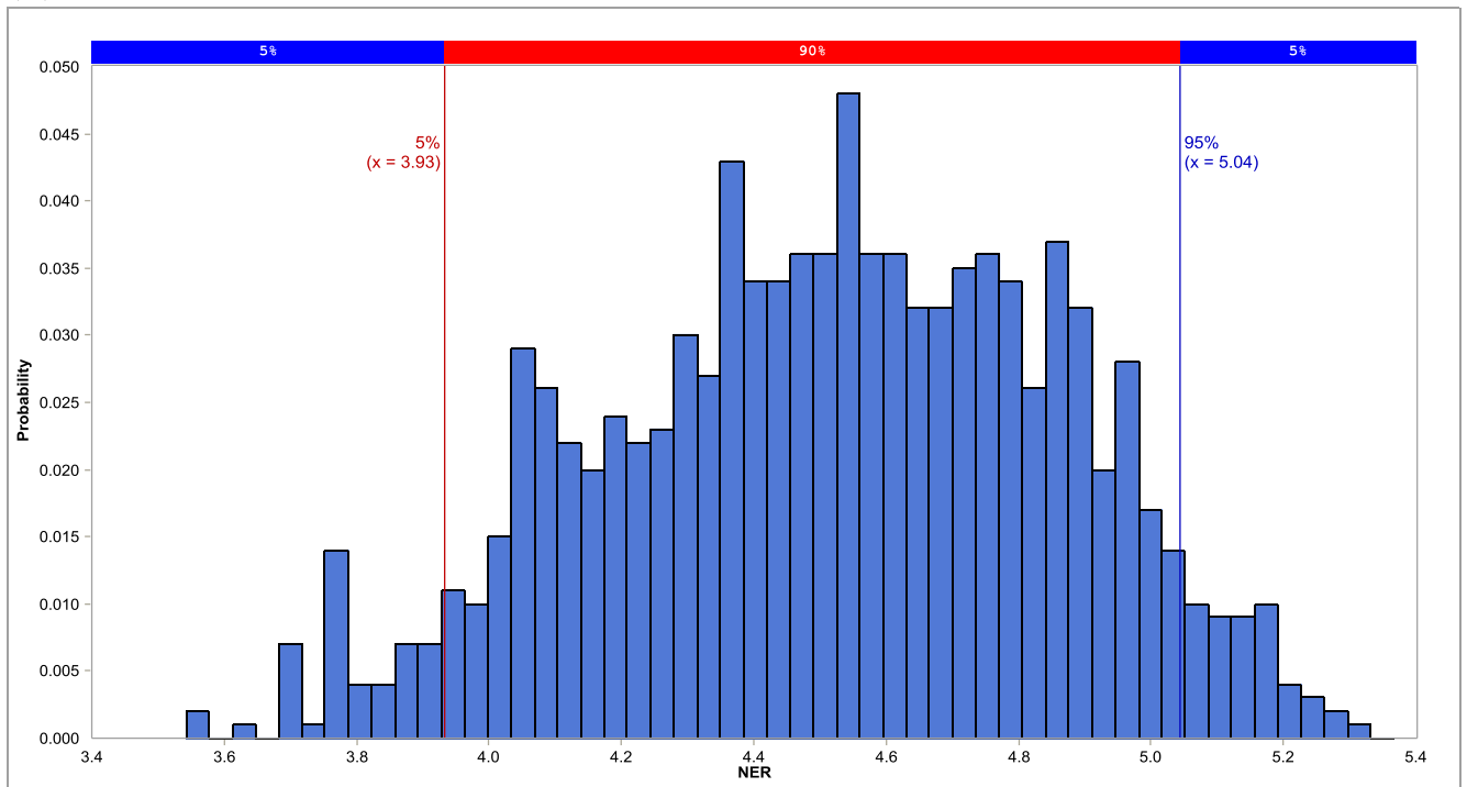
Fig. 6. Model uncertainty analysis of (A) steam pretreated Pellet NER and (B) Regular pellet NER.
