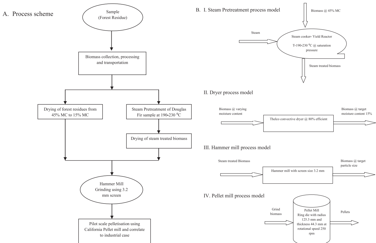
Fig. 2. Process scheme and model assumptions used in Aspen PLUS for: (A) Regular & Steam Pretreated Pellet Production; and (B) Unit Operation assumption [28].
