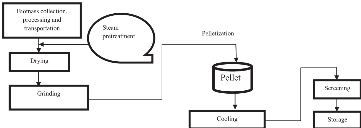
Fig. 1. Production chain of regular pellets and steam-treated pellets.
