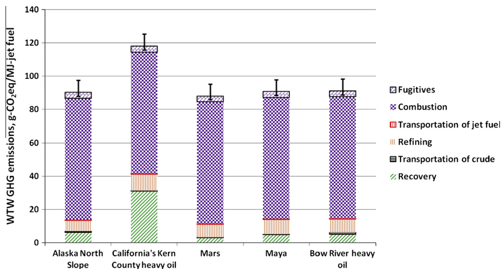
Fig. 10. Life cycle WTW GHG emissions for jet fuel.
