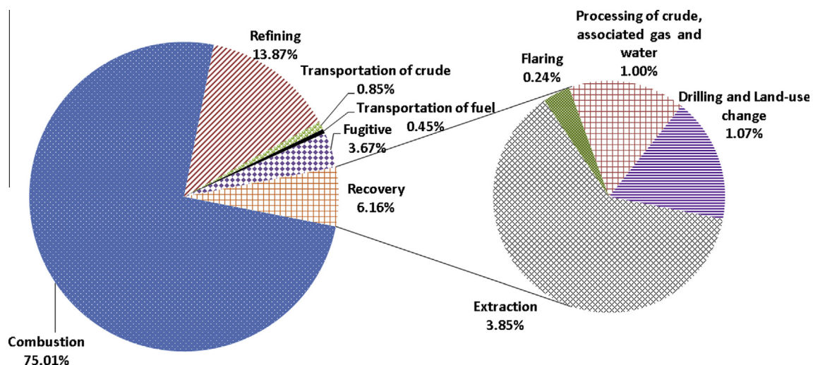
Fig. 11. Percentage contribution of GHG emissions for gasoline obtained from Alaska North Slope.
