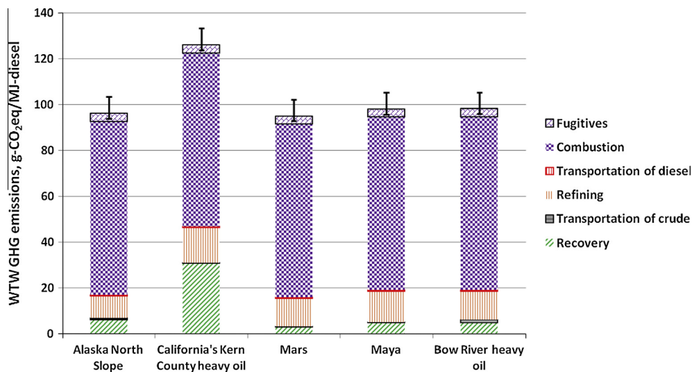
Fig. 9. Life cycle WTW GHG emissions for diesel.
