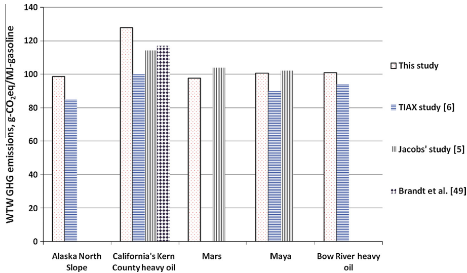
Fig. 12. Comparison of WTW GHG emissions for gasoline with existing literature.
