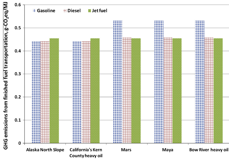
Fig. 7. GHG emissions from the transportation of finished fuels.
