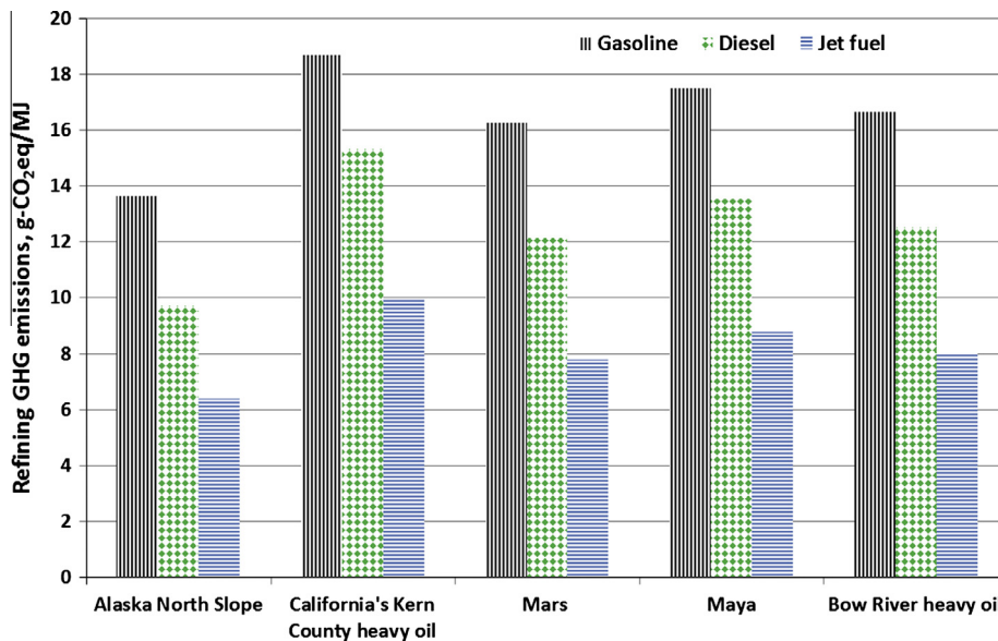
Fig. 5. GHG emissions for transportation fuels based on sub-process level allocation: mass-based.
