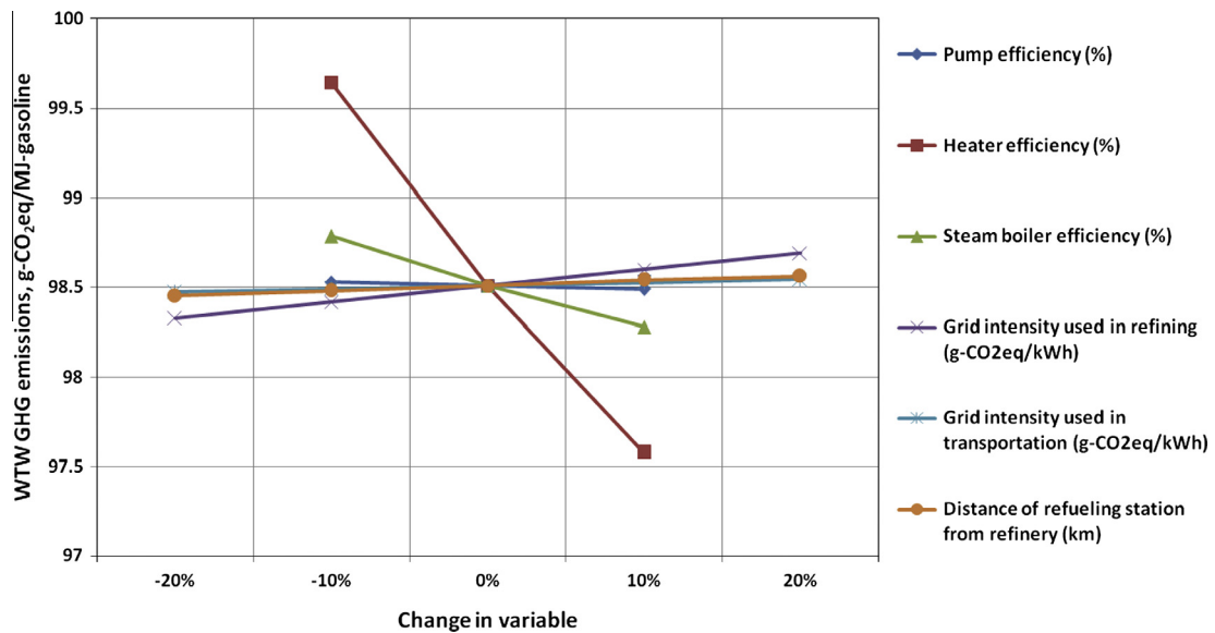
Fig. 13. Sensitivity analysis of total WTW GHG emissions for gasoline derived from Alaska North Slope.
