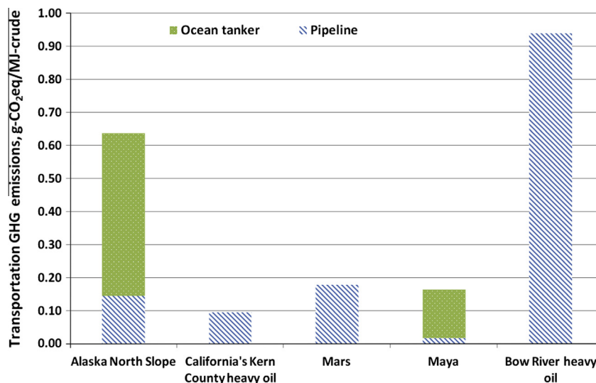
Fig. 6. GHG emissions from pipeline and ocean tanker transportation.
