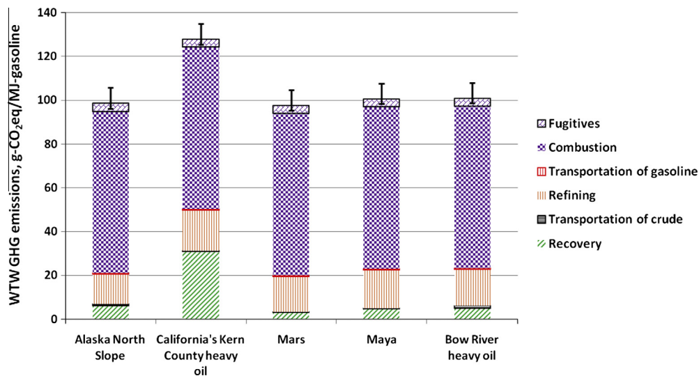
Fig. 8. Life cycle WTW GHG emissions for gasoline.
