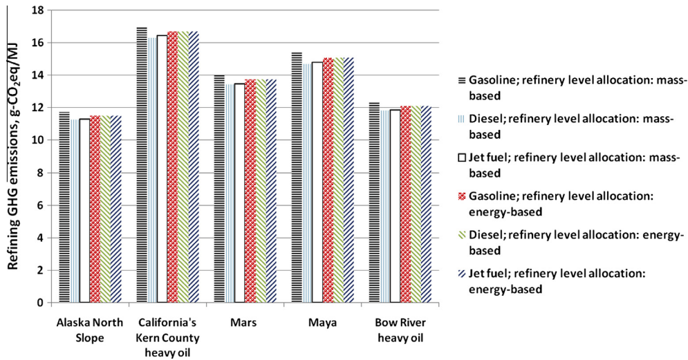
Fig. 4. GHG emissions for transportation fuels based on refinery level allocation.
