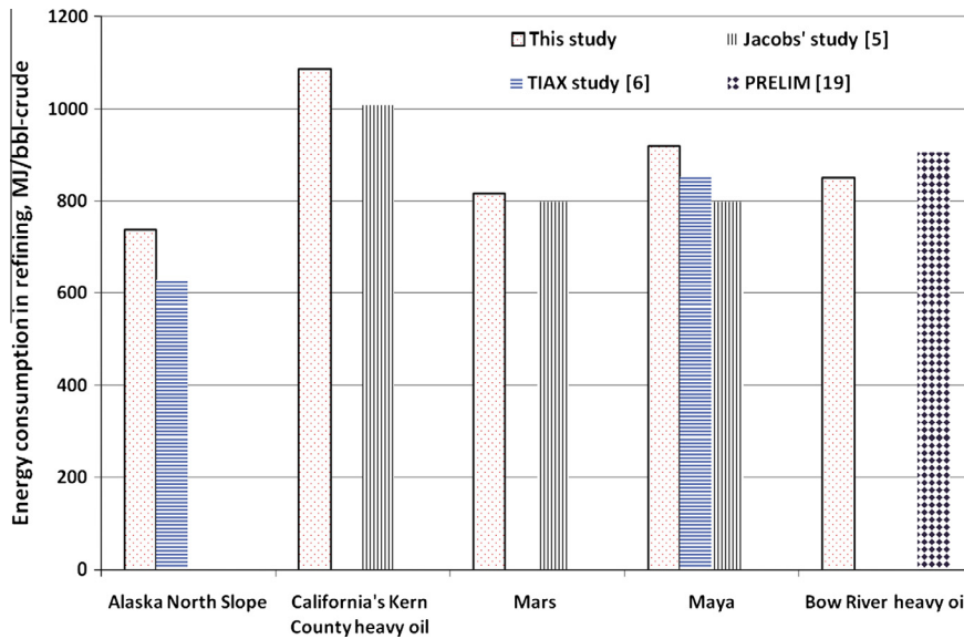
Fig. 3. Comparison of this study’s energy consumption results with existing data.
