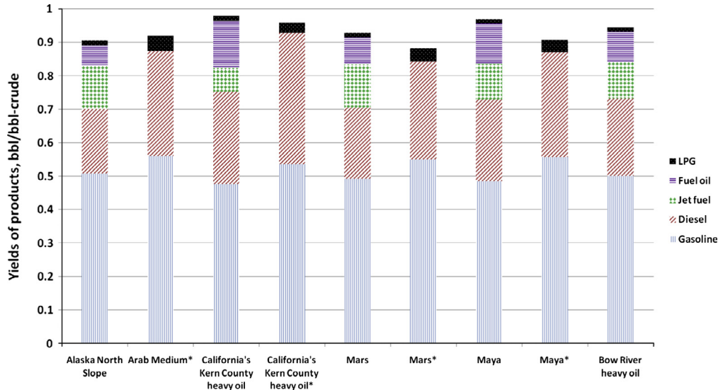
Fig. 2. Yields of products from the refining of crudes.
