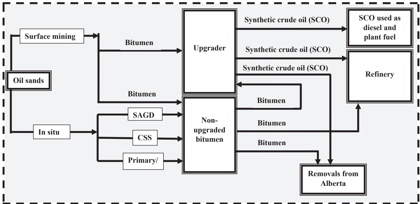
Fig. 2. System boundary of unit operations and production pathways of Alberta oil sands.
