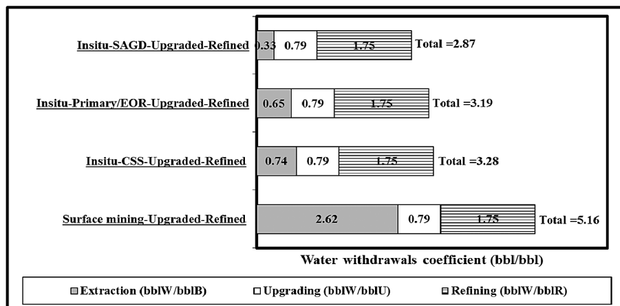
Fig. 4. Water withdrawals coefficients for the complete life cycle of Alberta oil sands.
