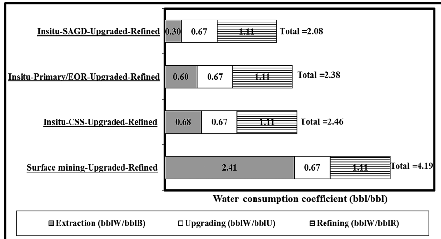
Fig. 3. Water consumption coefficients for the complete life cycle of Alberta oil sands.
