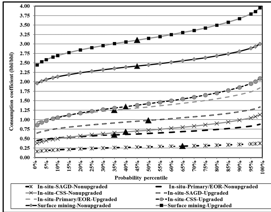
Fig. 6. Distribution of water consumption coefficients for refined oil sands pathways. ▲ The most likely value and the accompanied probability is shown in the graph for each pathway.
