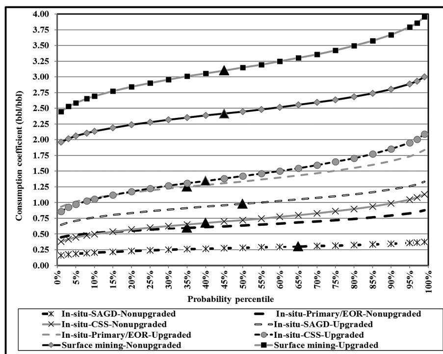
Fig. 5. Distribution of water consumption coefficients for unrefined oil sands pathways. ▲ The most likely value and the accompanied probability is shown in the graph for each pathway.
